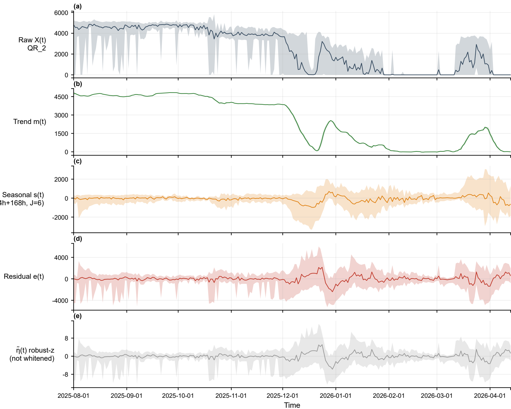
Full-span daily overview — QR_2 (recycle, min) [2025-08-01~2026-04-13]
